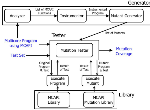
Fig. 4. Overview of Mutation Coverage Tool Architecture
